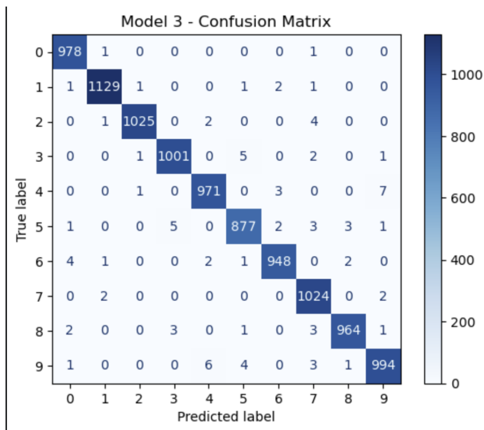
Figure 8: Confusion matrix of the best-performing CNN model evaluated using the MNIST testing dataset.
