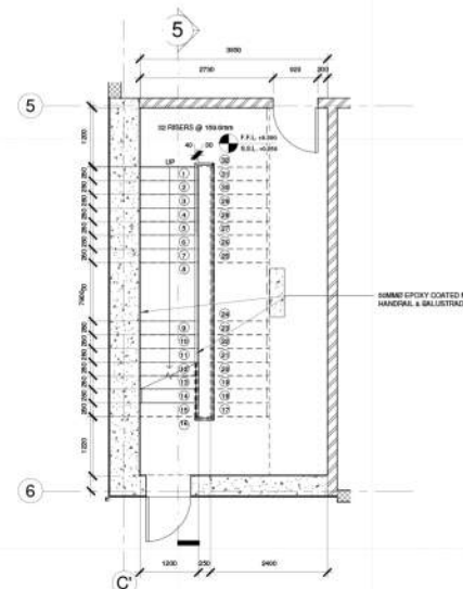
2 Staircase-Ground Floor 1 : 50
