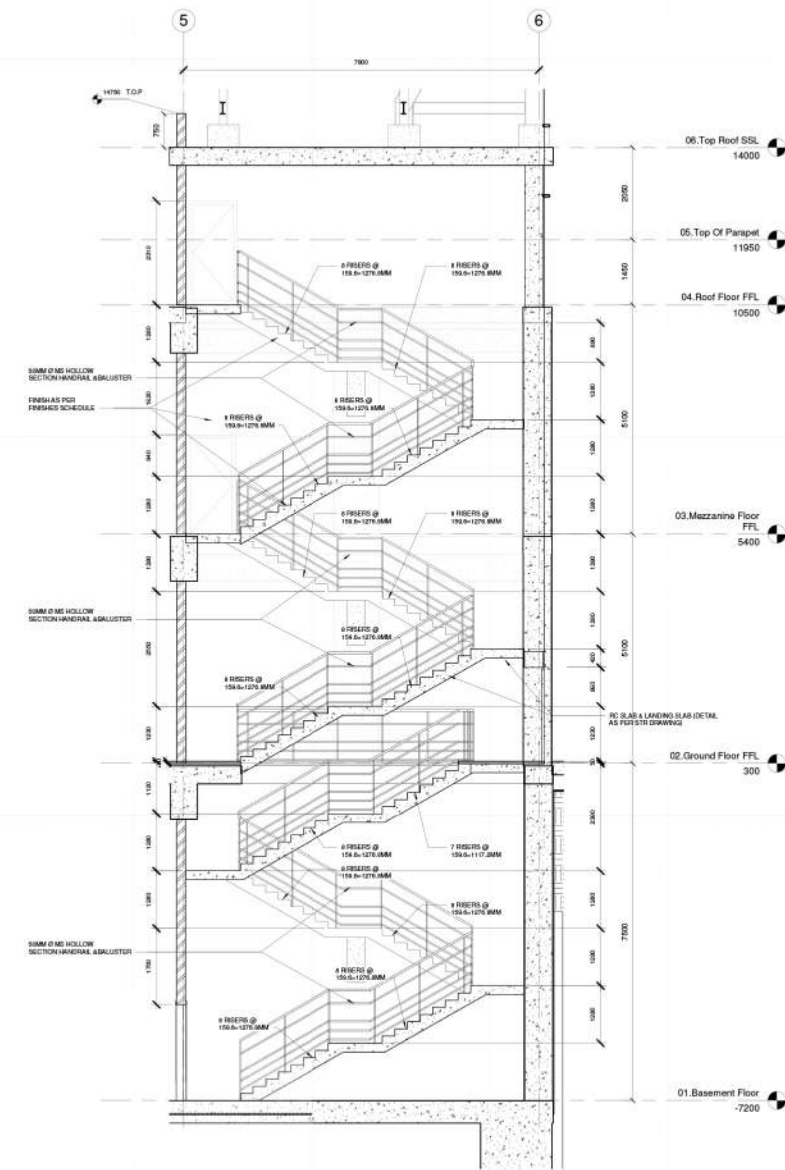
5 STAIRCASE SECTION 1 : 50
