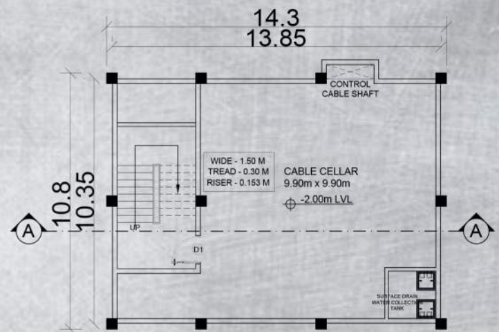
CABLE CELLAR PLAN
