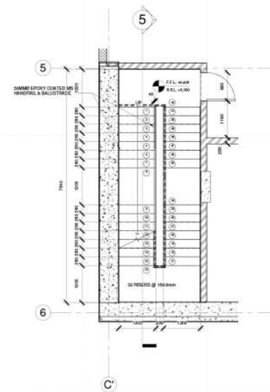
3 Staircase-Mezzanine Floor 1 : 50
