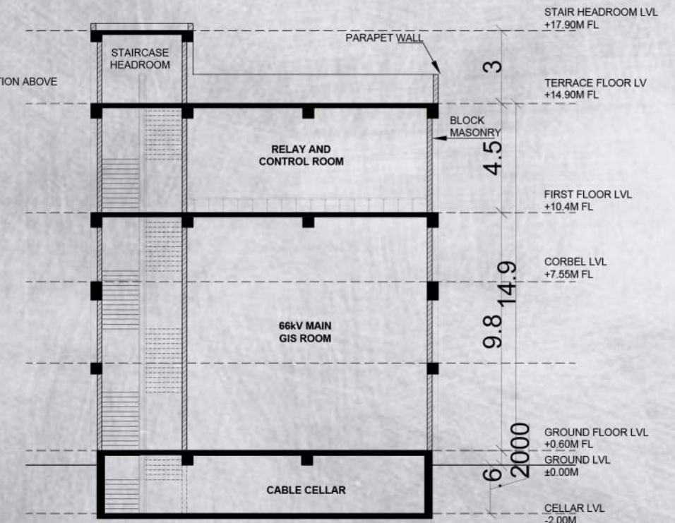
SECTION - AA
