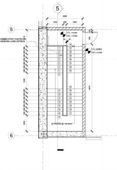
4 Staircase-Roof Plan 1 : 50
