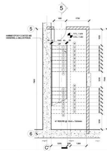
1 Staircase-Basement Floor 1 : 50
