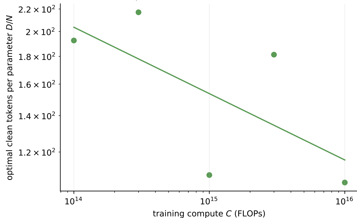
Optimal data ratio ( D/N \propto C^{-0.122} )
