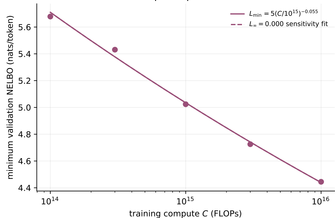
Compute-optimal loss
