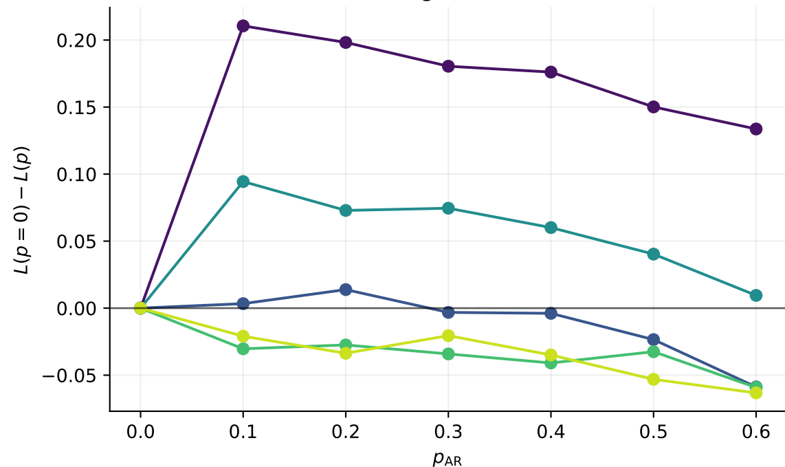
Best nonzero curriculum gain
