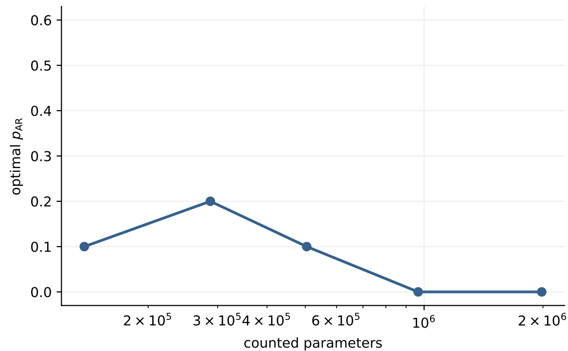
Best curriculum fraction
