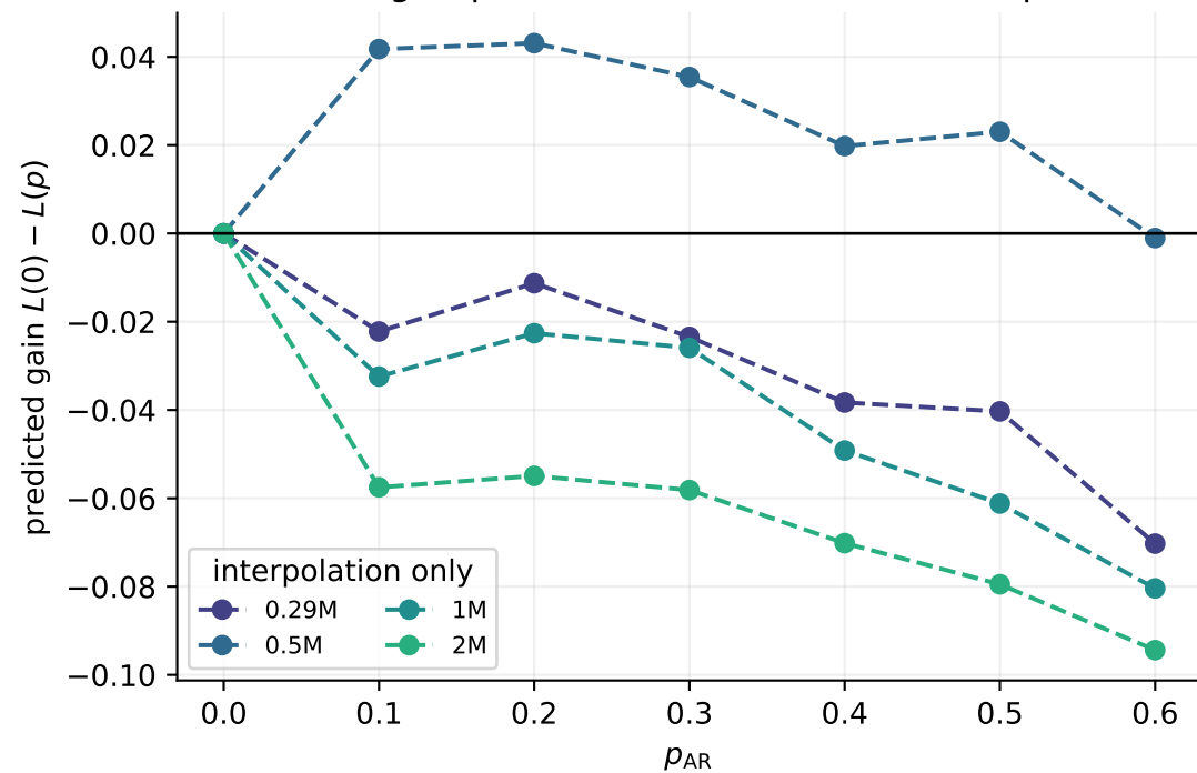
Old-grid prediction at matched total steps
