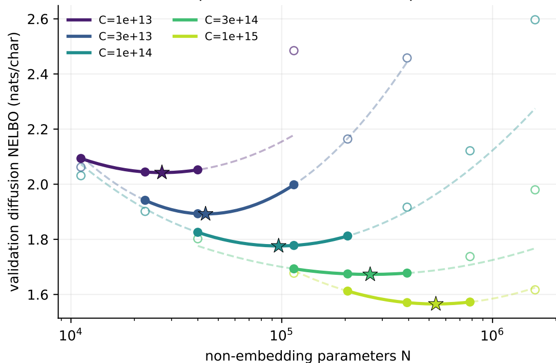
Optimal parameter-to-token ratio
