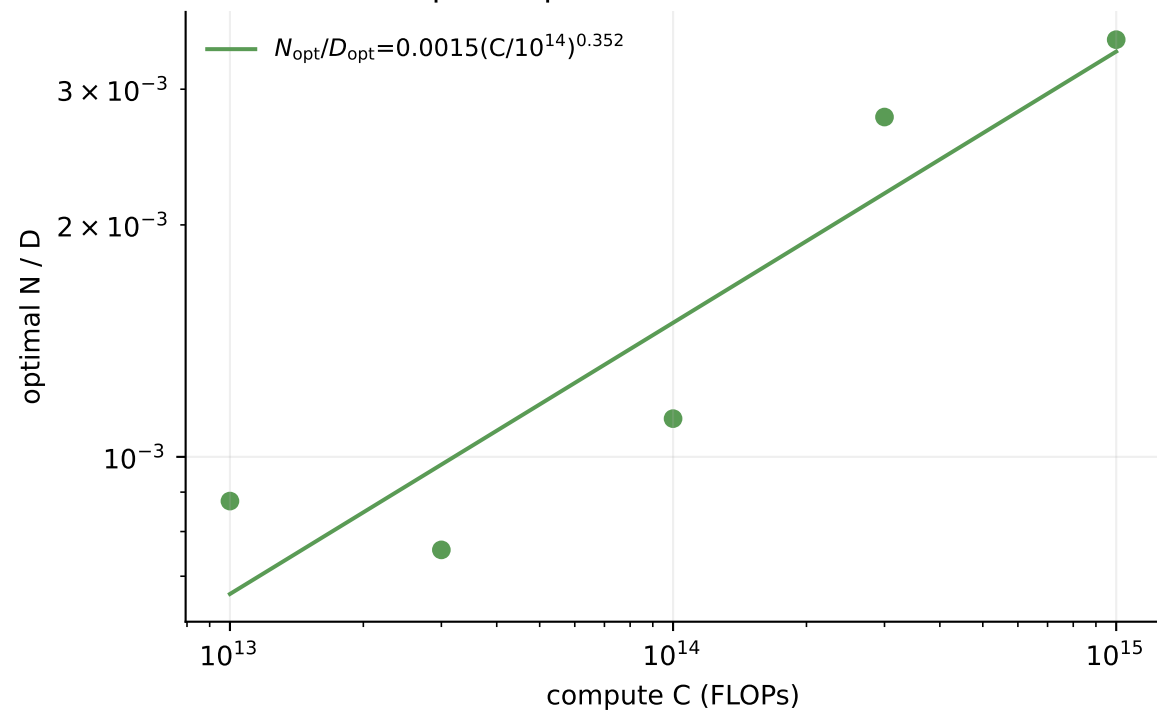
Optimal parameter-to-token ratio
