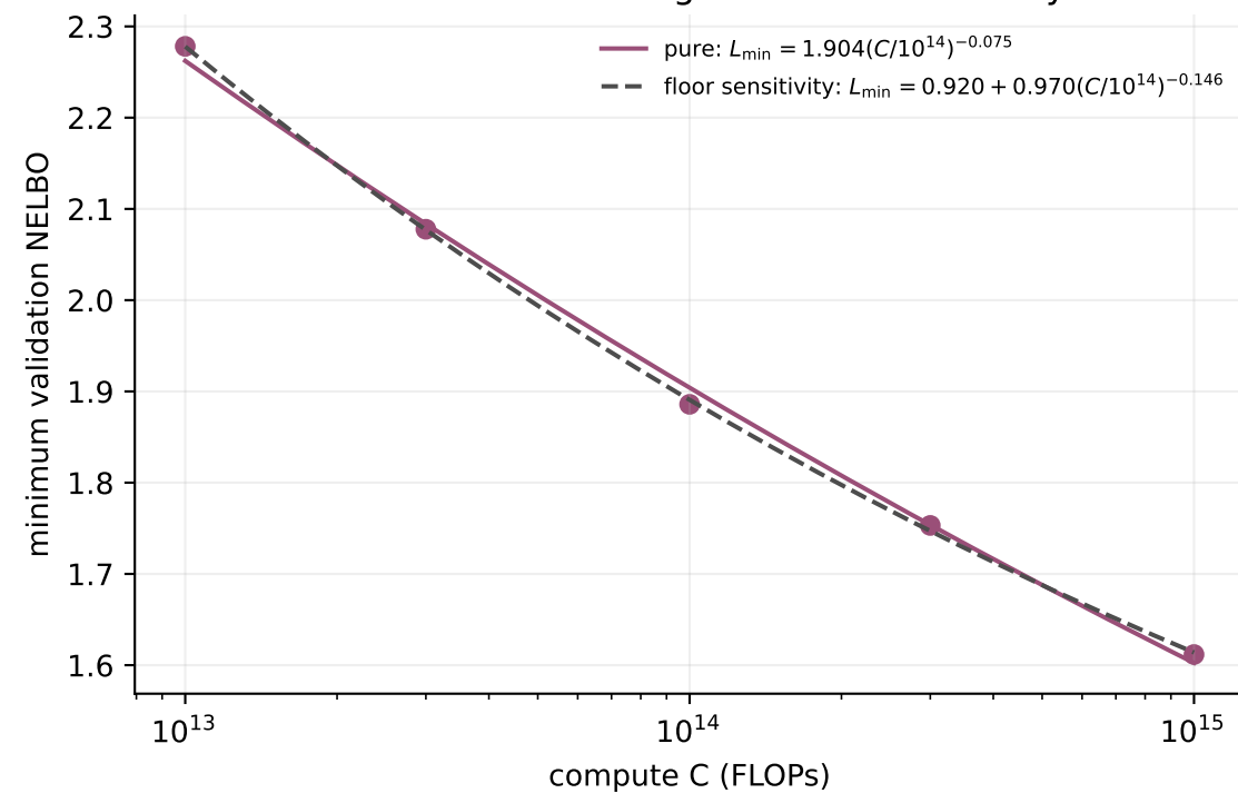
Minimum-loss scaling with floor sensitivity
