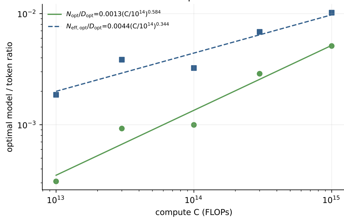
Counted and compute-effective ratios
