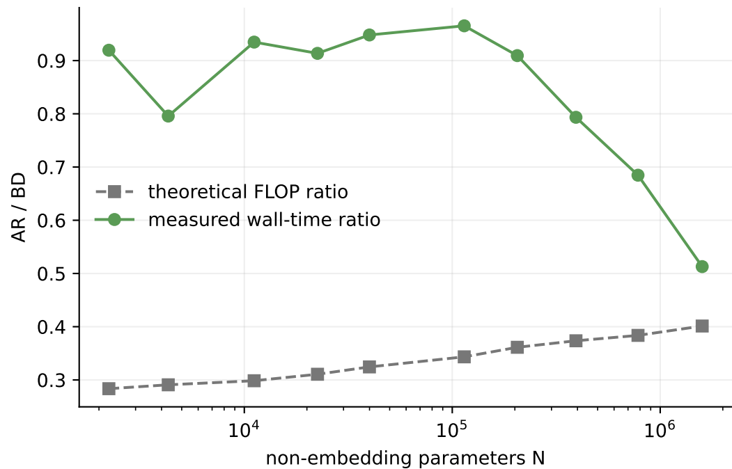
AR cost relative to block diffusion
