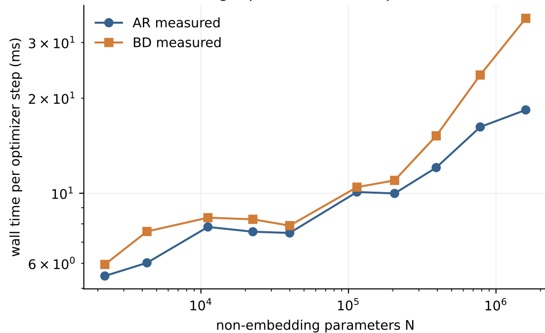
Single-process H100 step time
