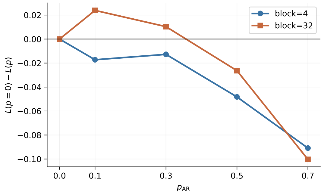
Curriculum gain within block size
