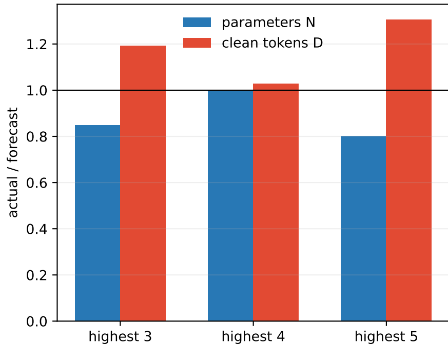
Chosen allocation versus rolling laws
