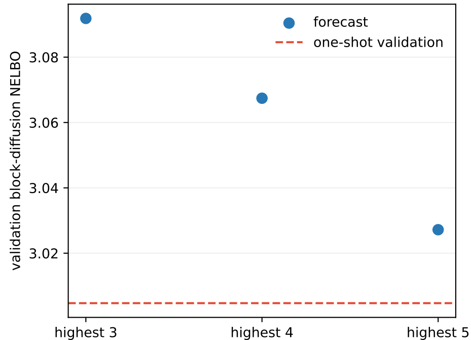
Loss forecast at 10^{19} FLOPs
