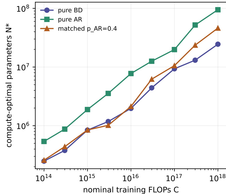
Optimal model size
