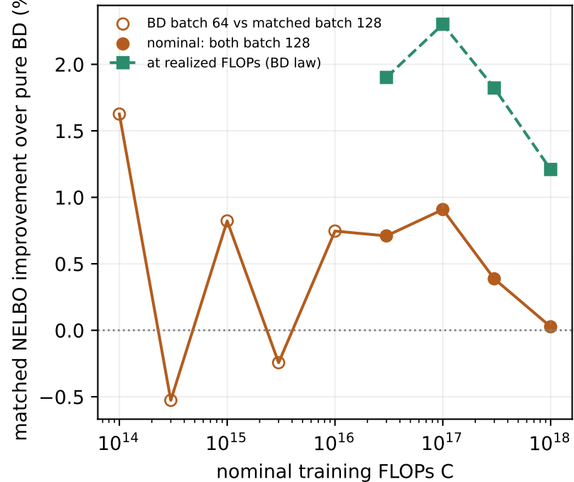
Matched-step frontier effect
