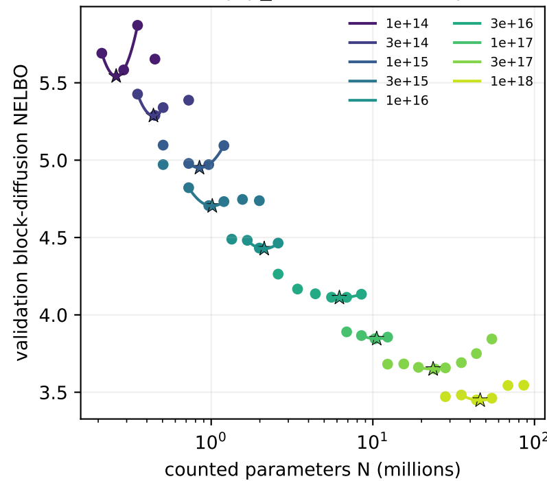
Matched-step p_AR=0.4 IsoFLOP profiles
