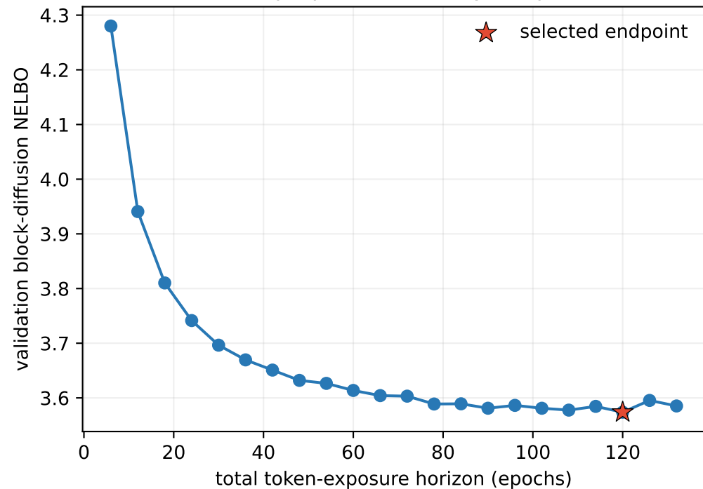
Full BD: proportional decay endpoints
