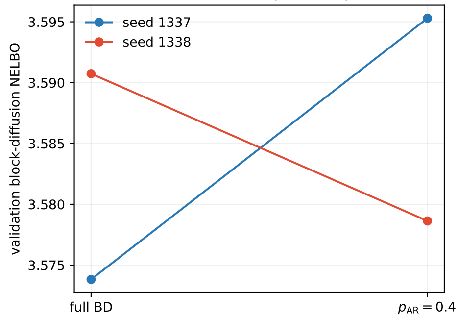
Untuned WD=0.1 paired repeats
