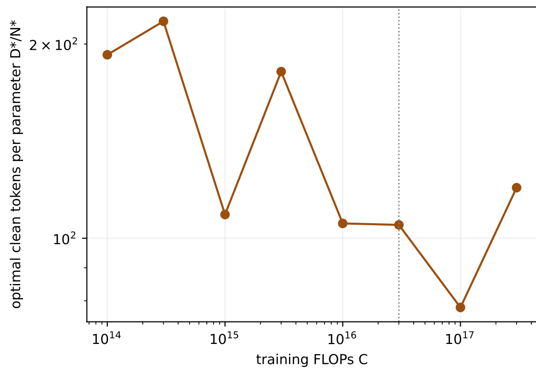
Allocation ratio
