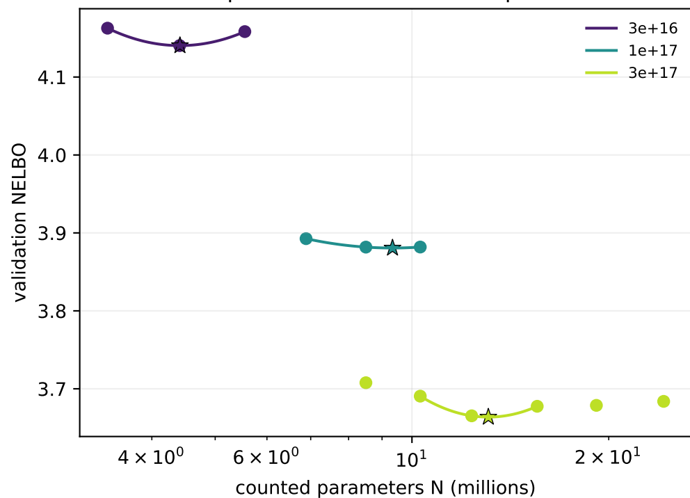
Allocation ratio
