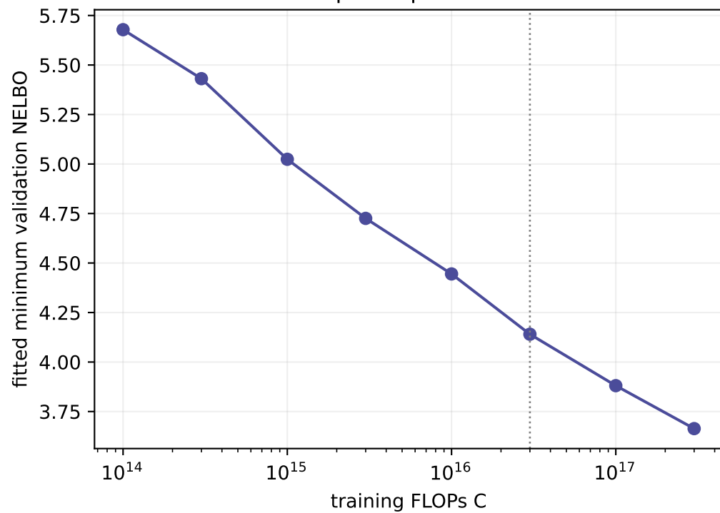
Compute-optimal loss
