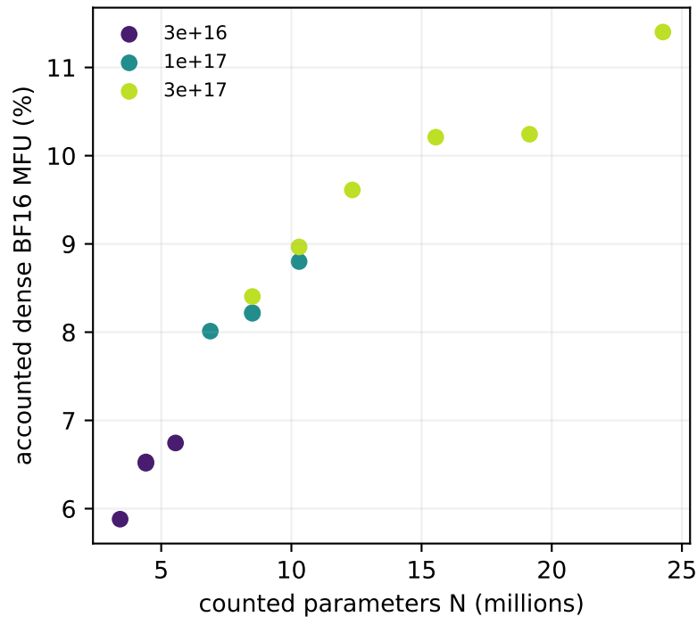
One-GPU H100 efficiency
