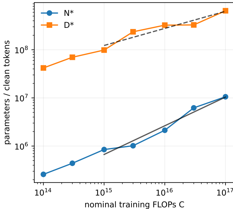
Compute-optimal allocation
