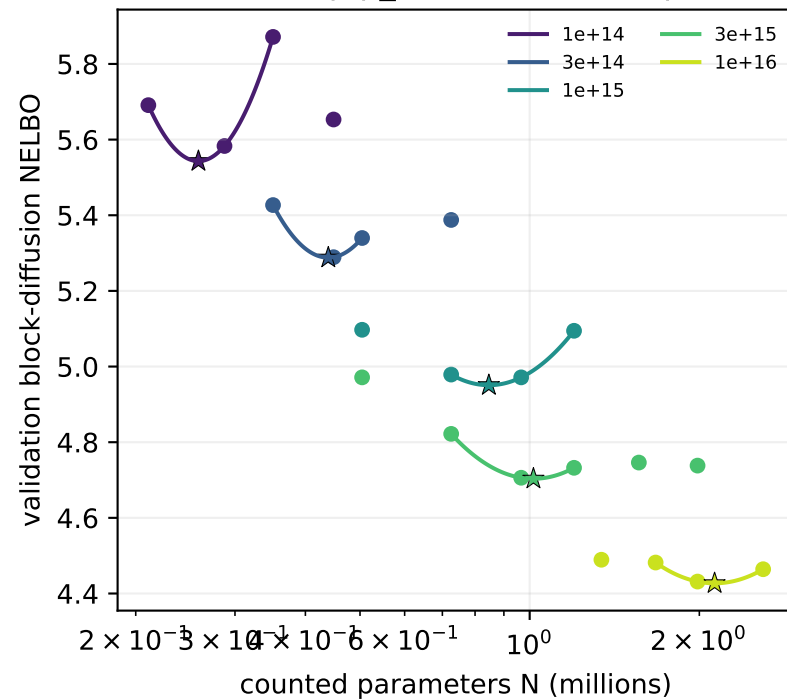
Matched-step p_AR=0.4 IsoFLOP profiles
