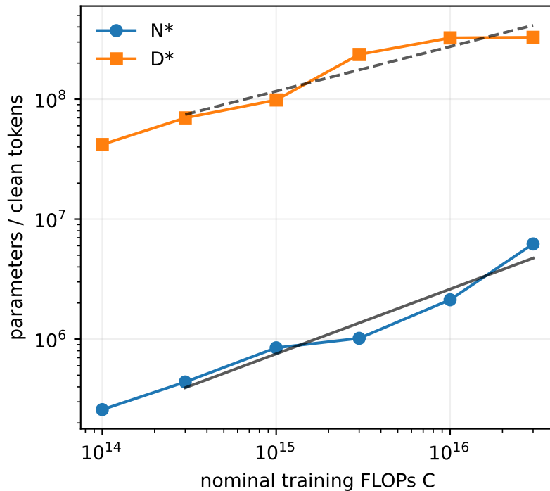
Compute-optimal allocation
