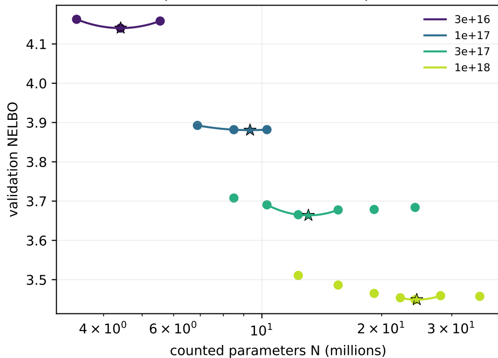
Allocation ratio
