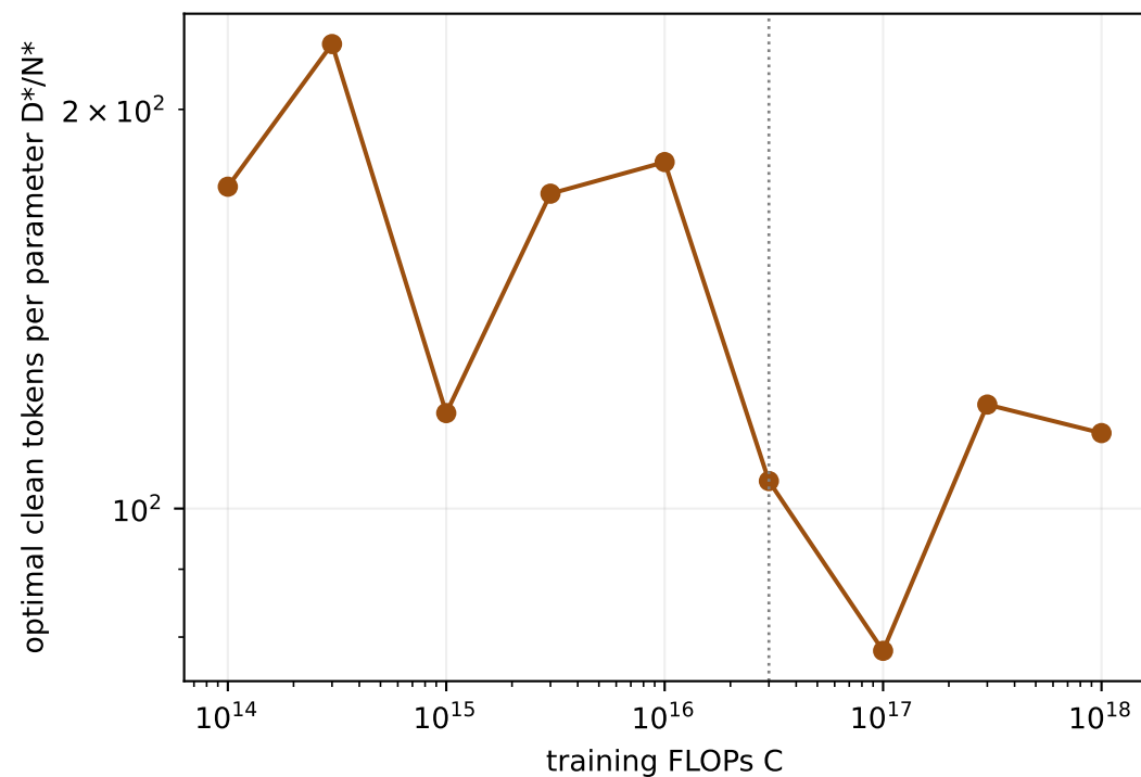
Allocation ratio
