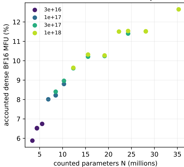
One-GPU H100 efficiency
