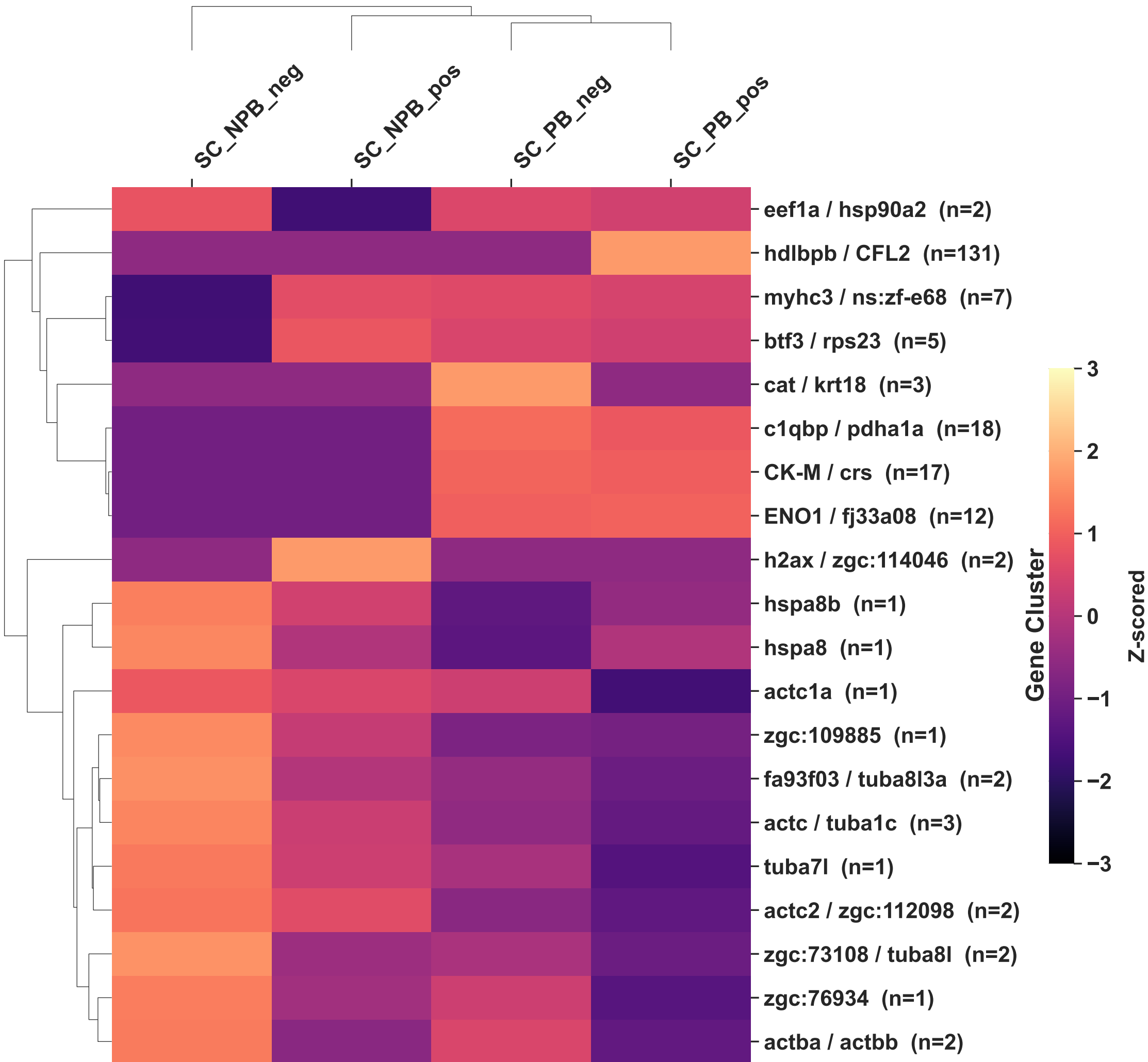
All Proteins - SC - KMeans Gene Clusters (k=20)
