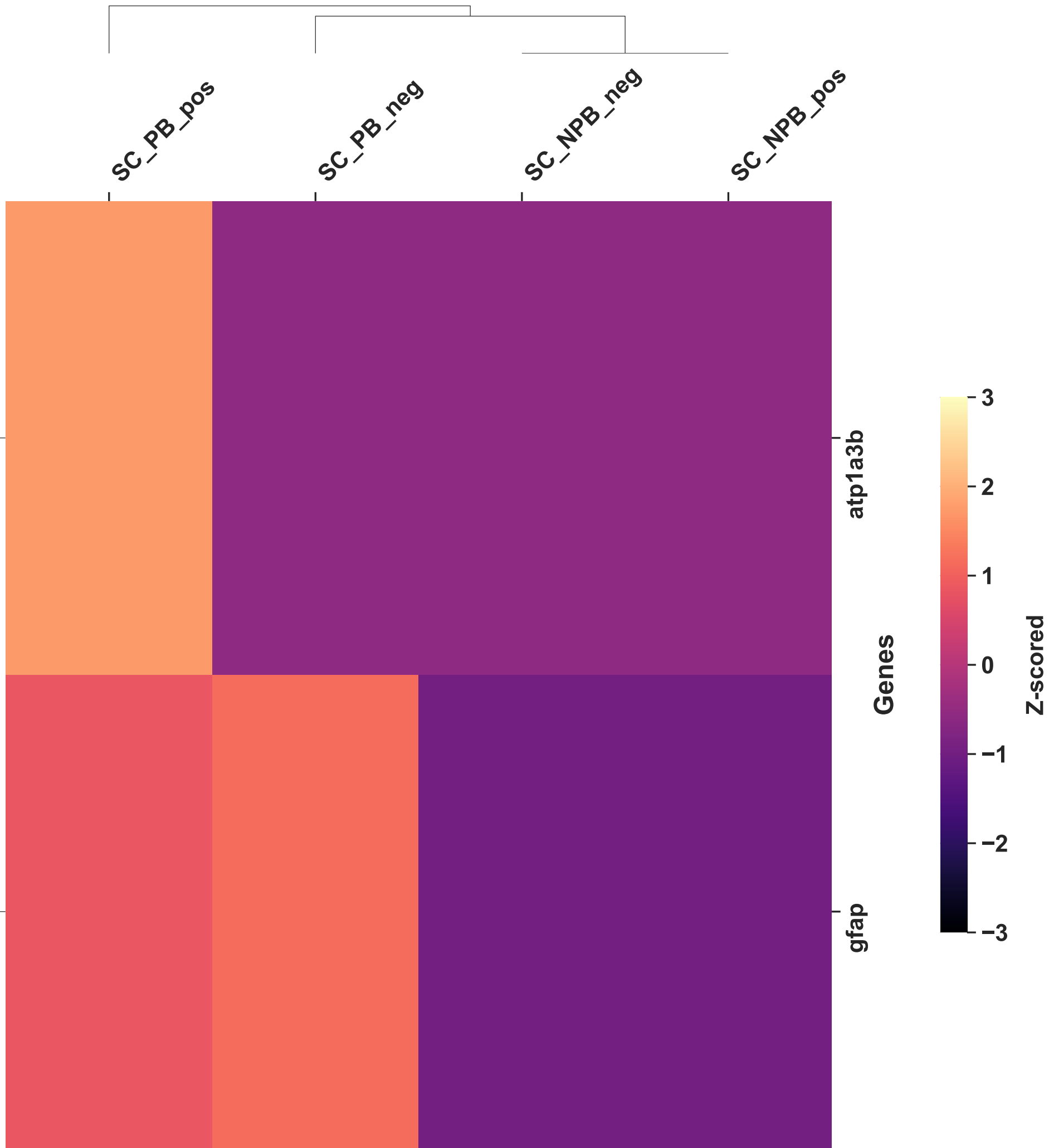
SC Genes (3-6 dpf subset) - All Samples
