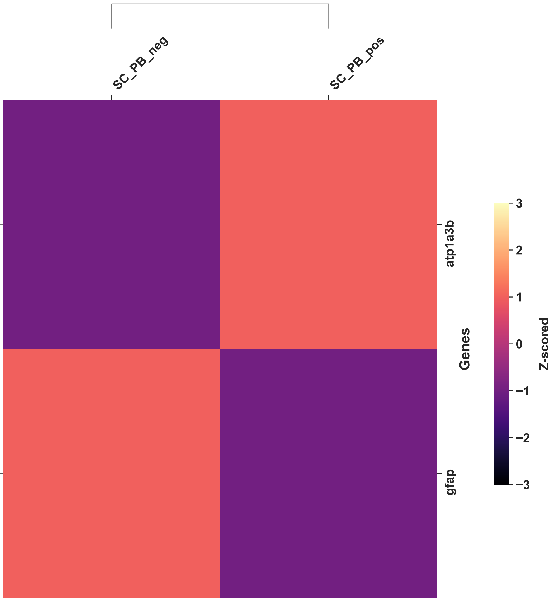
SC Genes (3-6 dpf subset) - PB Only
