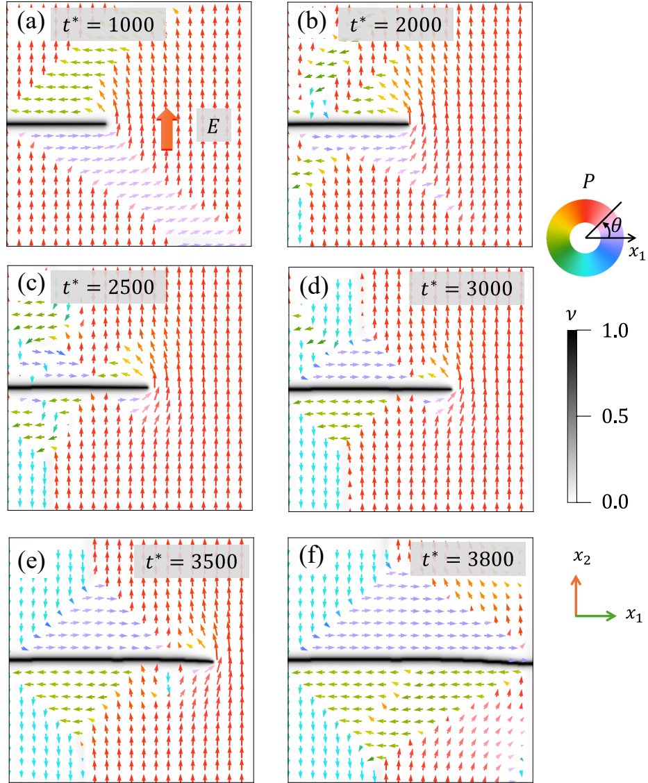
Figure 13: Evolution of polarization domain and the crack extension at moments t^* = 1000 , t^* = 2000 , t^* = 2500 , t^* = 3000 , t^* = 3500 , and t^* = 3800 under the applied electric field E_y^* = 1 , respectively. The flexoelectric effect is considered in this case.
