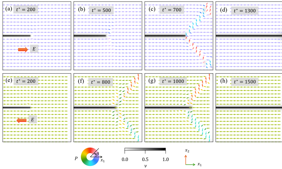
Figure S1: The temporal evolution of crack and polarization domain: (a)-(d) crack propagates along the polarization direction, (e)-(h) crack direction opposite to the polarization. The grayscale maps illustrate the spatial distribution of the fracture order parameter \nu . The arrows indicate the orientation and magnitude of the polarization vectors. The flexoelectric effect is considered in this figure.
