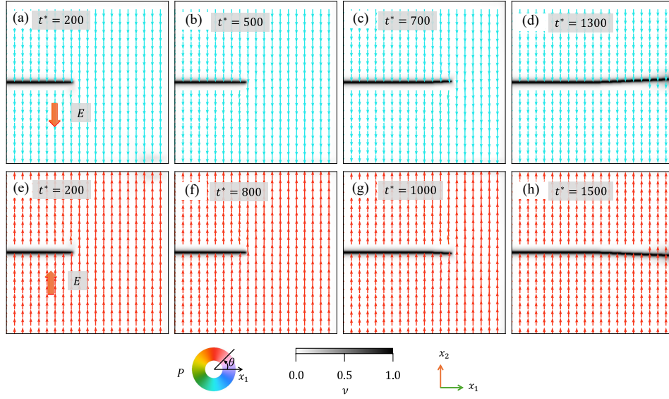
Figure S3: The temporal evolution of crack and polarization domain: (a)-(d) initial polarization is opposite to the x_2 -direction, (e)-(h) initial polarization is along the x_2 -direction.
