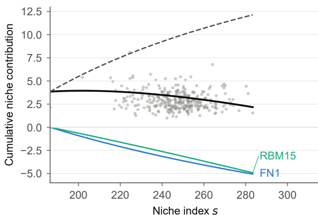
d SERPINE1 curve decomposition
