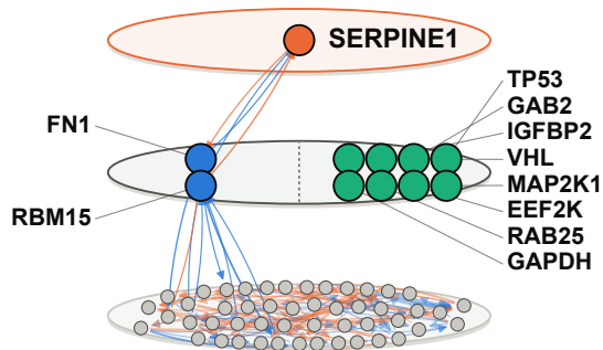
c SERPINE1 joint / conditional rank 2 / 2
