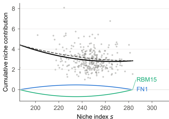
d SERPINE1 curve decomposition
