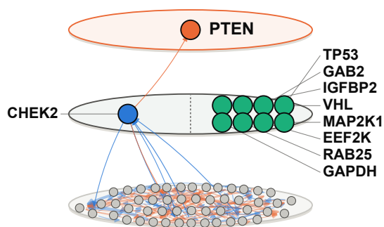
a PTEN joint / conditional rank 1 / 1
