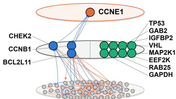
e CCNE1 joint / conditional rank 2 / 2
