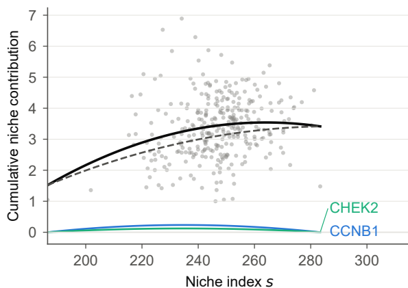
f CCNE1 curve decomposition
