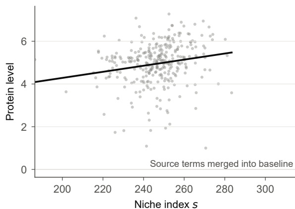
b PTEN zero-degree niche trend
