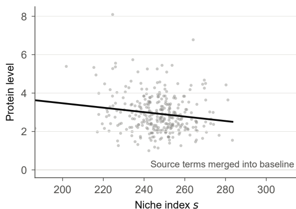
d SERPINE1 zero-degree niche trend
