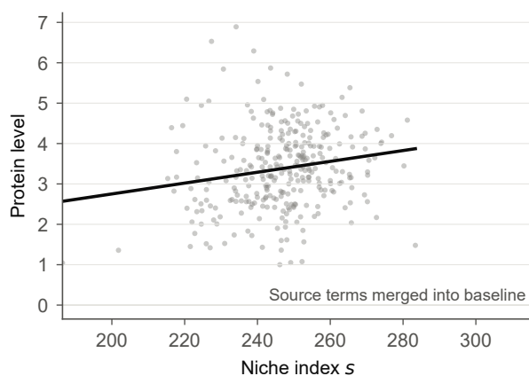
f CCNE1 zero-degree niche trend
