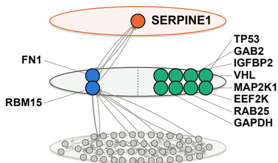
c SERPINE1 joint / conditional rank 2 / 2
