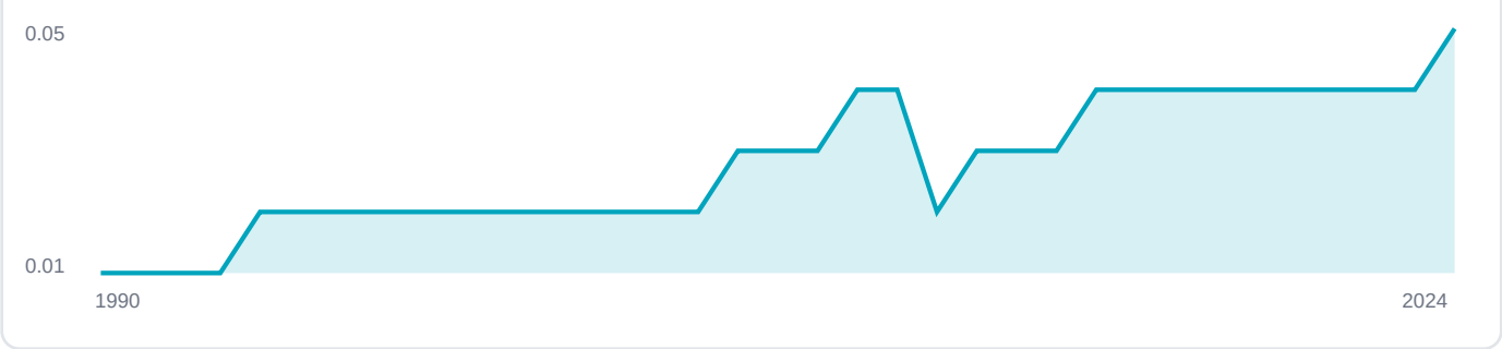
Transport CO2 emissions (Mt), 1990–2024, EDGAR
