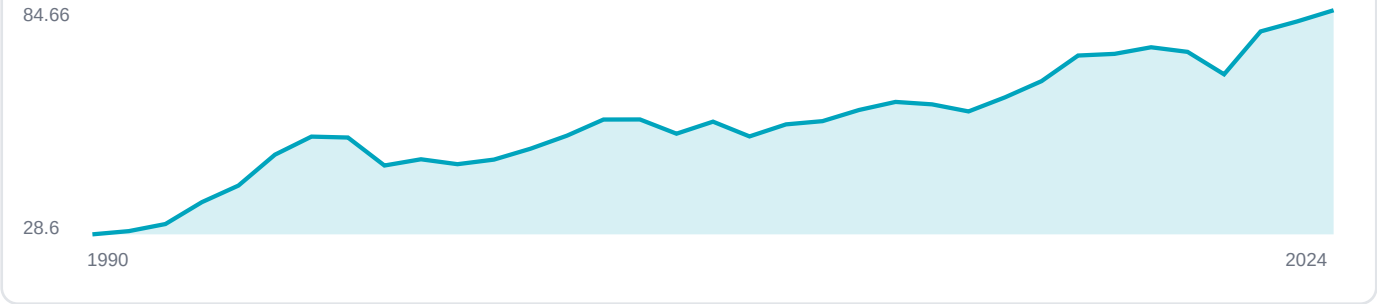
Transport CO2 emissions (Mt), 1990–2024, EDGAR
