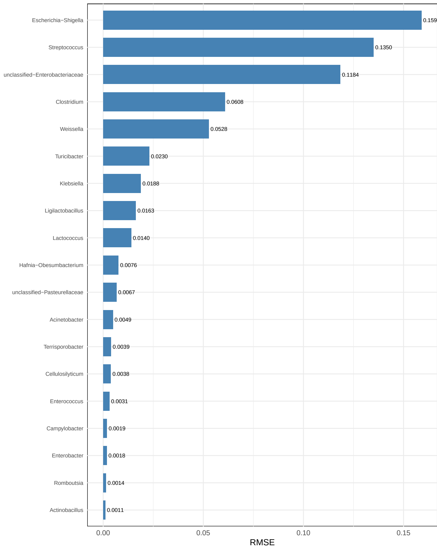
Per-Genus RMSE
