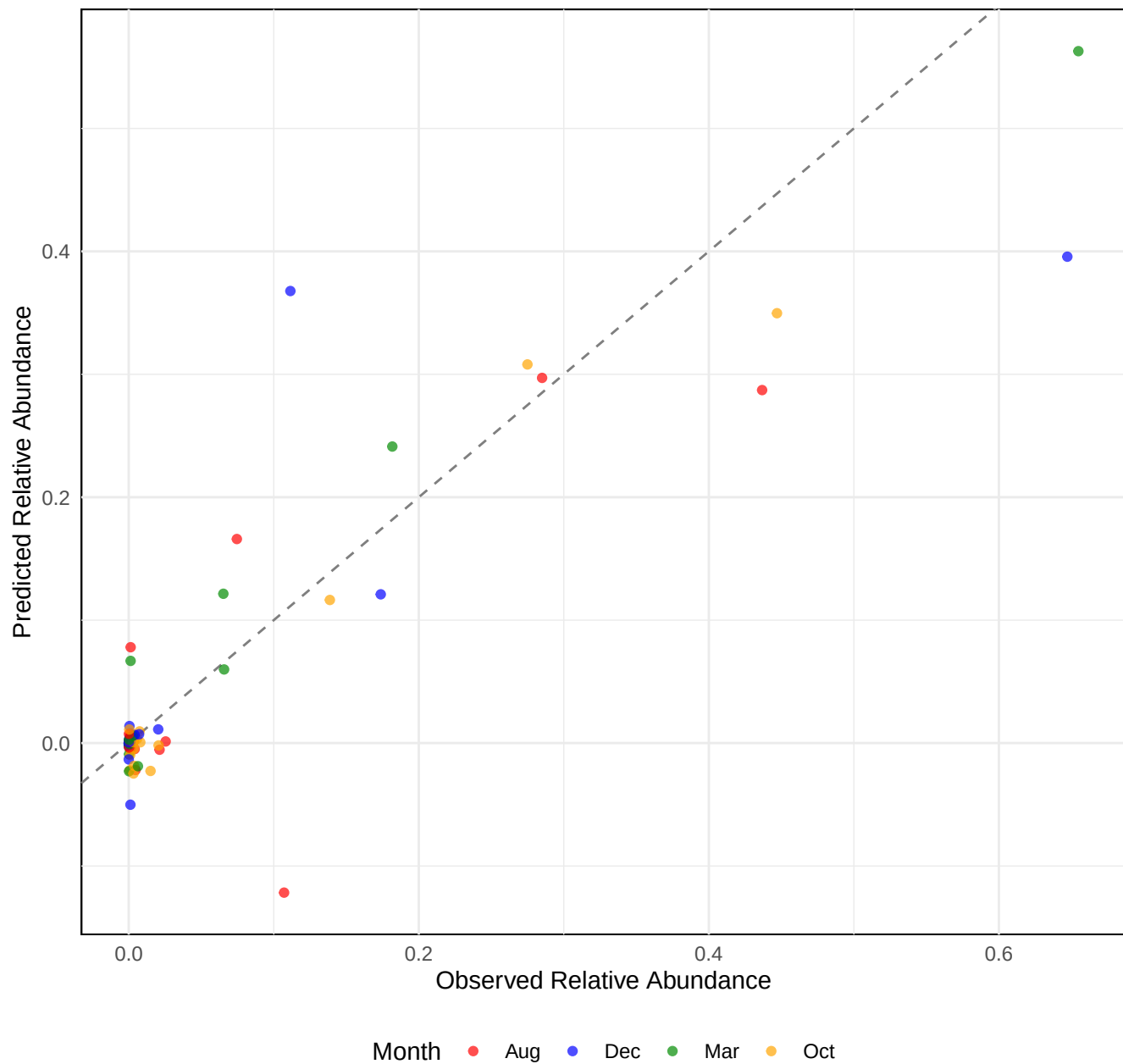
Model Validation: Predicted vs Observed
