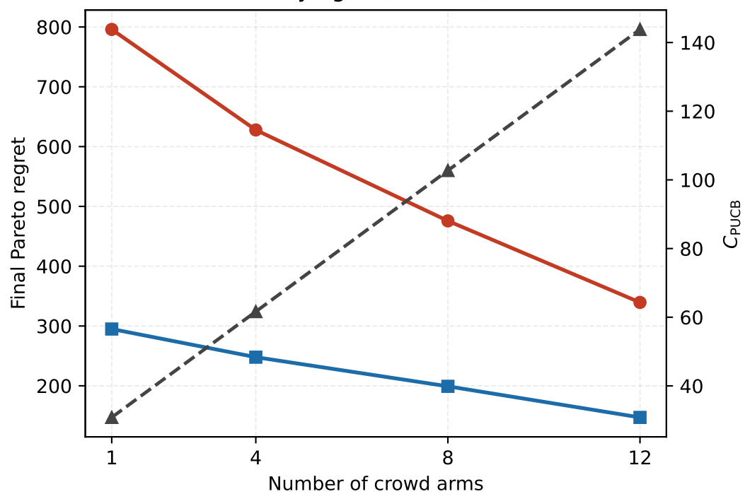
Varying m ( \delta = 0.02 )
