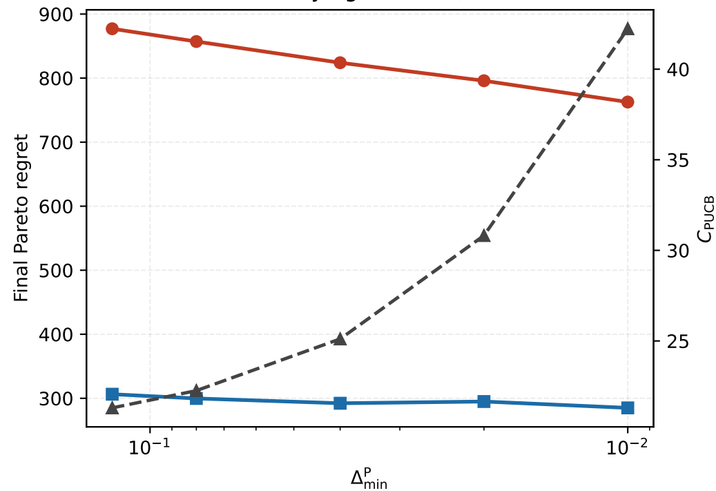
Varying \delta ( m = 1 )
