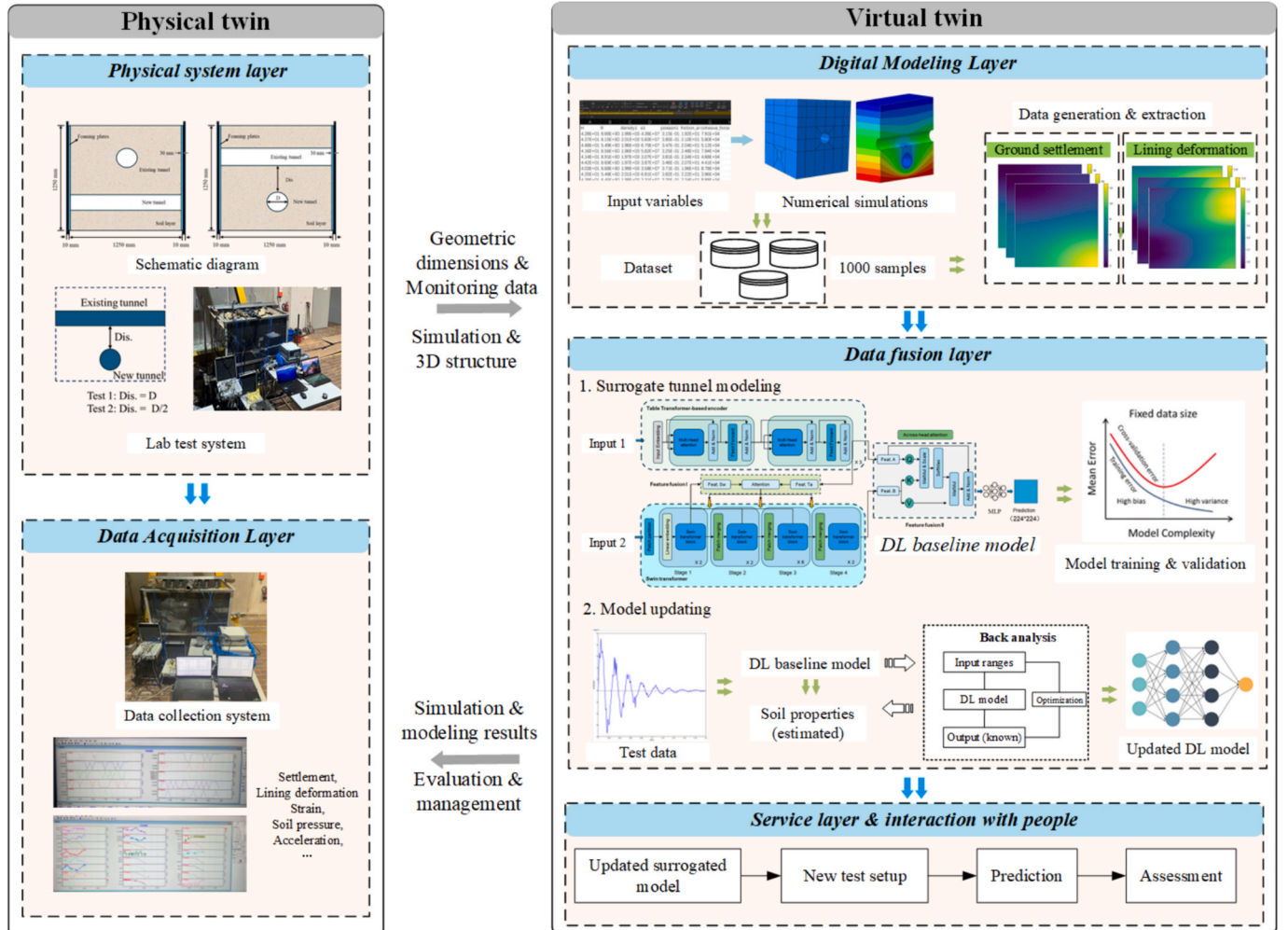
Fig. 1. The framework of the proposed method.
