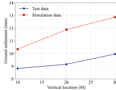
(b) Perpendicular to the excavation direction
