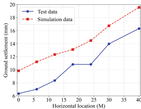
(a) Along the excavation direction
