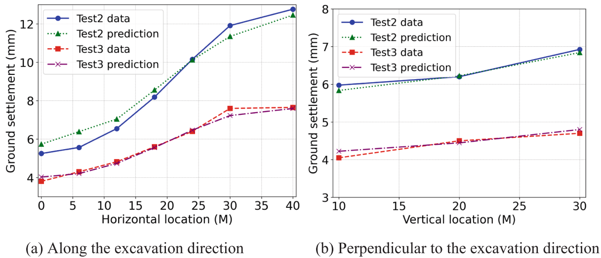
Fig. 16. Comparison of ground settlement data: test data vs. prediction results.
