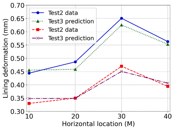
Fig. 17. Comparison of lining deformation data: test data vs. prediction results.
