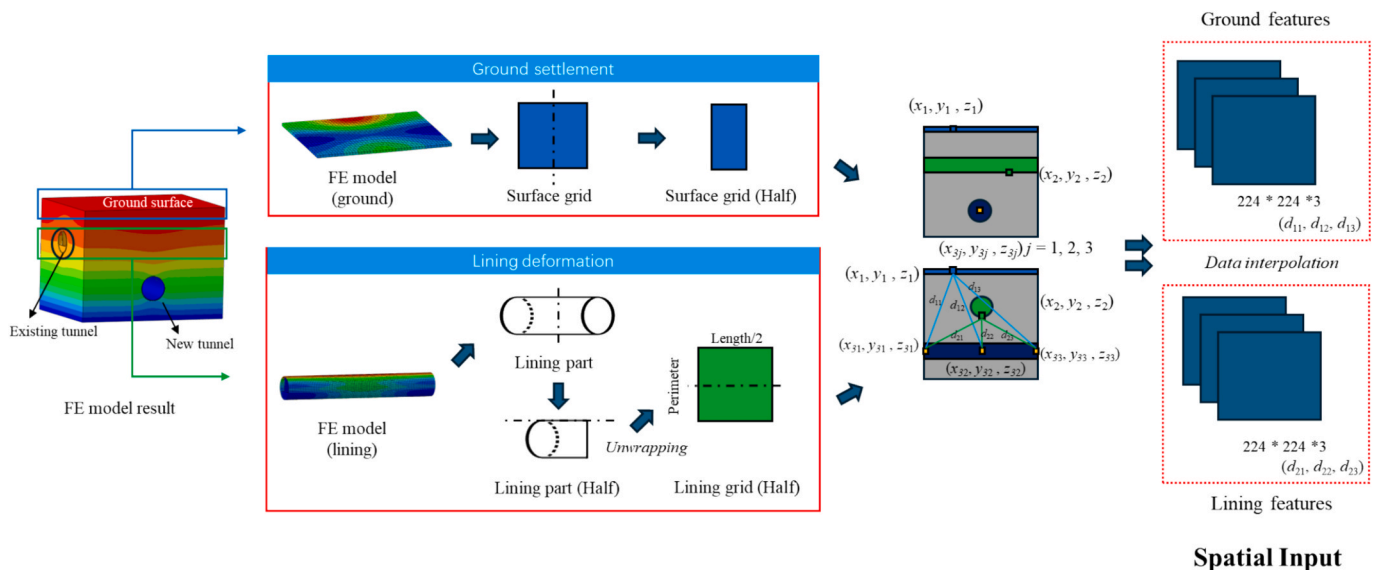
Fig. 2. Spatial information extraction.
