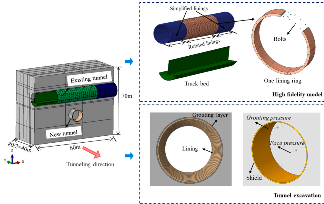
Fig. 8. The FE model in Abaqus.
