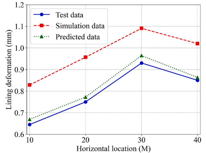
Fig. 15. Comparison of lining deformation data: test data vs. simulation and prediction results.
