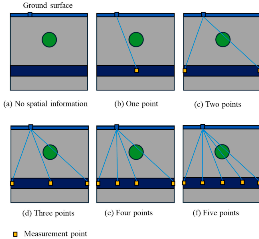
Fig. 11. Configurations of spatial measurement points used in the surrogate model.
