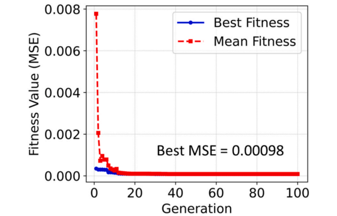
Fig. 14. GA convergence process during surrogate model updating for lining deformation.
