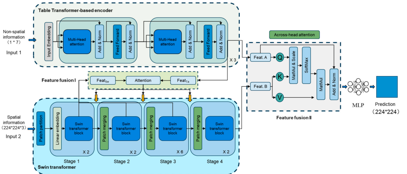
Fig. 4. DF-STTN for the surrogate model.
