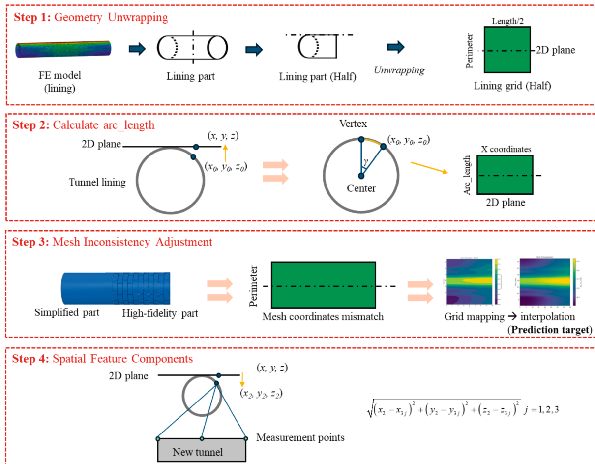
Fig. 3. Procedures of spatial information extraction of the lining deformation.
