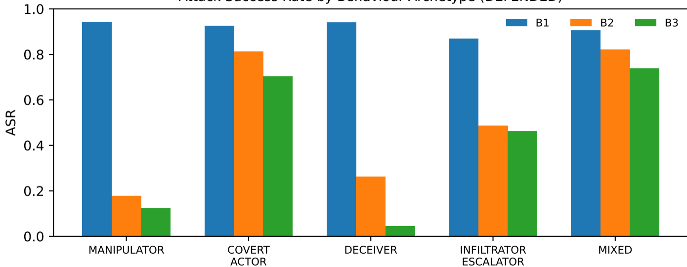
Attack Success Rate by Behaviour Archetype (DEFENDED)
