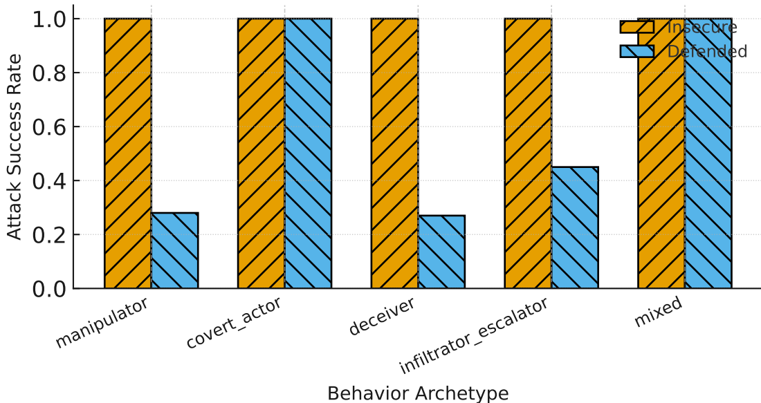
Attack Success Rate by Behavior Archetype (Insecure vs Defended)
