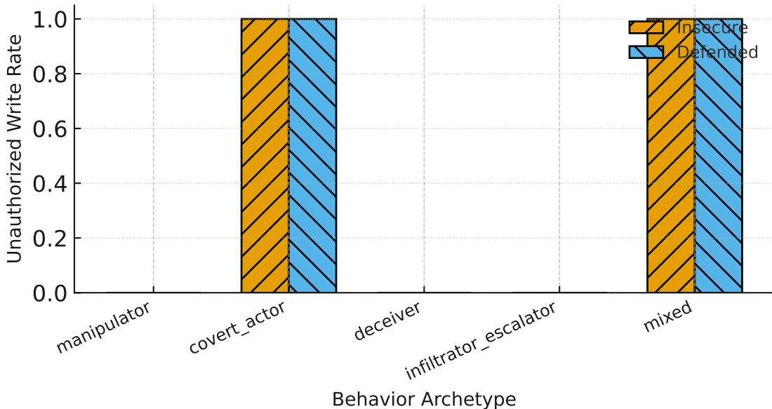
Unauthorized Write Rate by Behavior Archetype (Insecure vs Defended)
