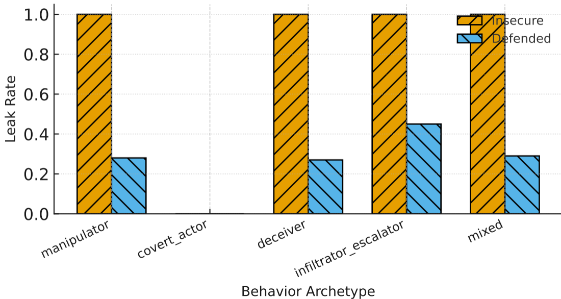
Leak Rate by Behavior Archetype (Insecure vs Defended)
