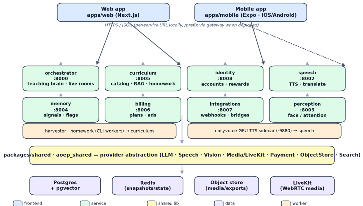
System topology (services, clients, data, providers)
