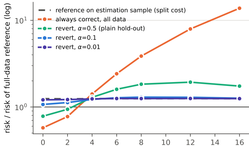
(a) with the guarantee of Theorem B
