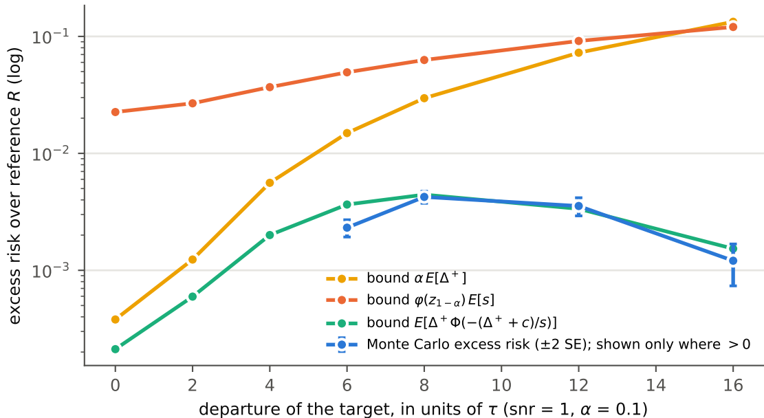
Do no harm: excess risk of the reverting estimator vs. Theorem B
