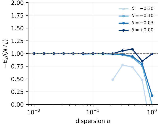
Error against the crossing term NT_u (Prop. 3)
