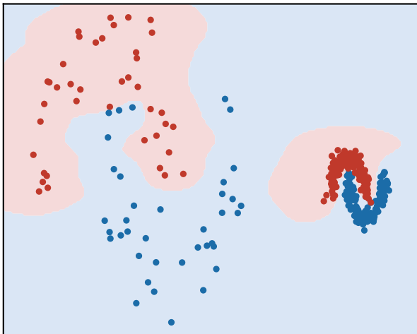
checker_2scale / rbf {'C': 10.0, 'gamma': np.float64(3.411)}
