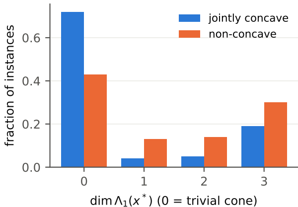
N = 3 players, 100 + 100 games
