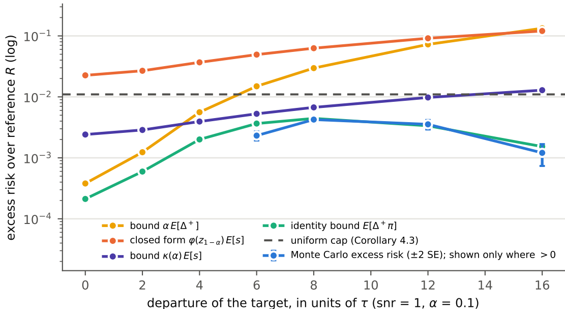
Do no harm: excess risk of the reverting estimator vs. Theorem 4.2
