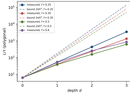
Figure 1: Polygonal L/\tau against depth for the default family (solid) and the conditional bound 2\pi\Lambda^d with c = 1/2 (dashed, f \leq 1/2 ).
