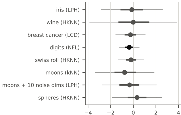
primary comparison
