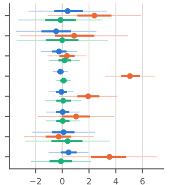
ablations
