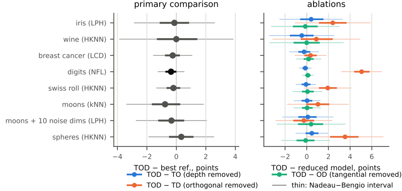
Figure 2: Left: TOD minus the best reference per dataset (C1). Right: the three ablations (C2). Thick segments: bootstrap 95% intervals; thin segments: intervals with the Nadeau–Bengio variance; black (left) marks a bootstrap interval excluding zero.
