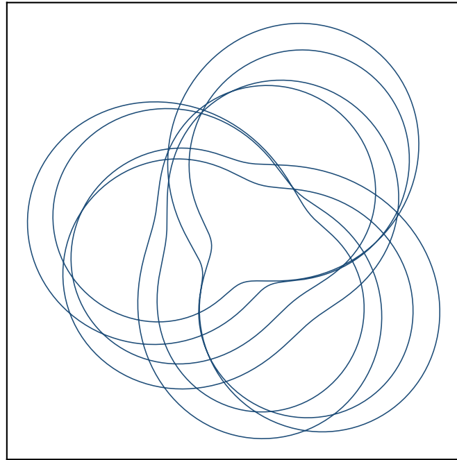
K_3 (projection to xy ), N = 8192
