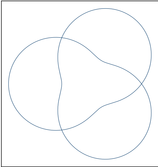
K_1 (projection to xy ), N = 2048
