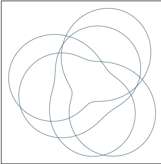
K_2 (projection to xy ), N = 4096
