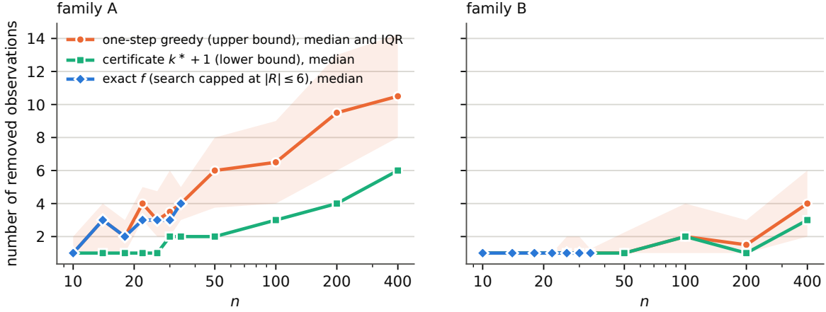
Figure 2: Bracketing the fragility number at large n (rule C): median one-step greedy witness size (upper bound, with interquartile range) and median certified lower bound k^* + 1 from Proposition ??, per family; exact medians from E4 where available.
