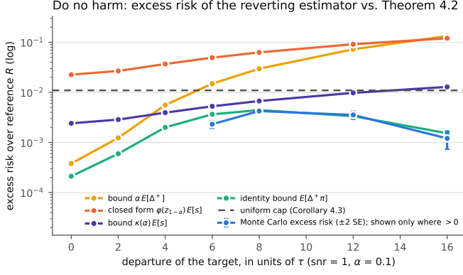
Figure 2: Excess risk over R on the departure sweep ( \alpha = 0.1 ) against the bounds of Theorem 4.2, the closed form \varphi(z)\mathbb{E}[s] and the cap of Corollary 4.3 (dashed). The identity bound \mathbb{E}[\Delta^+\pi] is nearly attained where the excess is positive; at \kappa = 8 the \kappa -bound is 0.0067 against an excess of +0.0042; at \kappa = 16 the cap (0.0110) is below the \kappa -bound (0.0129).
