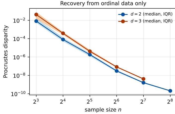
Figure 1: E2. Median and interquartile range of the Procrustes disparity of the ordinal reconstruction as a function of n , for d = 2 and d = 3 .
