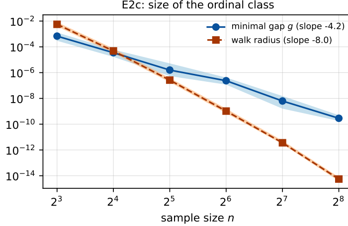
Figure 2: E2c. Median and interquartile range of the minimal gap g and of the walk radius against n ( d = 2 ).
