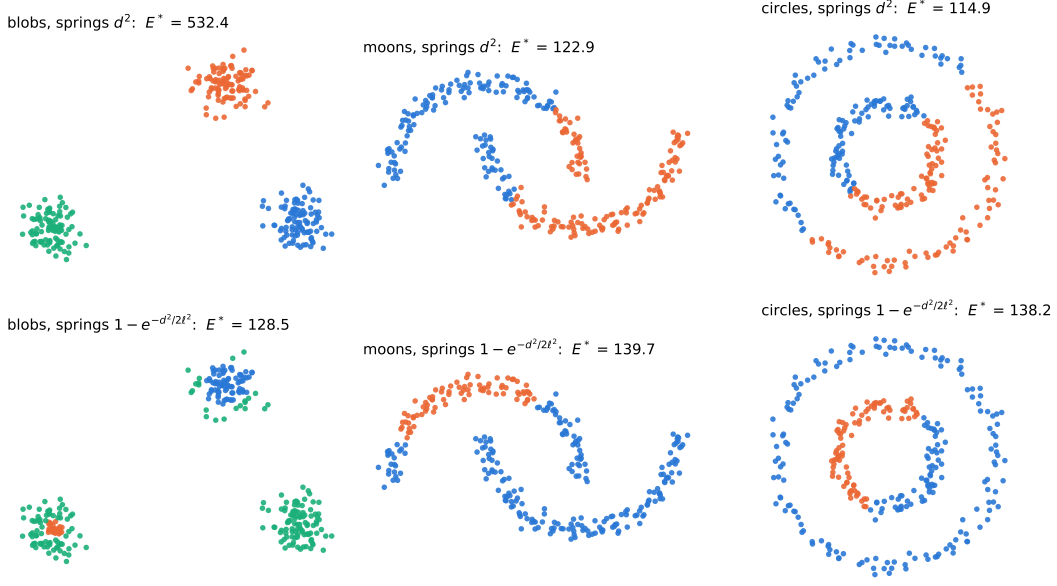
Figure 2: Best partitions found by spring relaxation on the synthetic sets for Hooke and saturating springs. Each is, by Theorem ??, a kernel k -means optimum of the linear and Gaussian kernels respectively, with the same value; the figure illustrates the family, it does not evaluate it.
